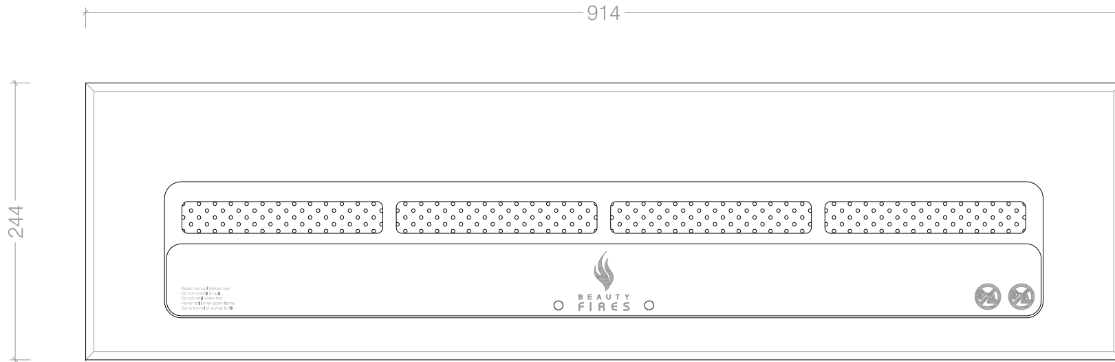
Top View
