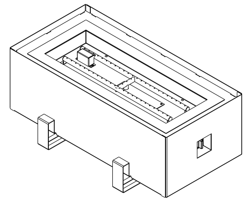
Complete Unit: Gas Rectangular Firepit - 900mm Gas Firepit Burner - 800mm
