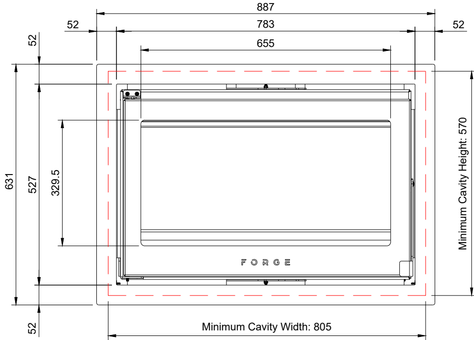
Forge F80 Double Sided Insert
